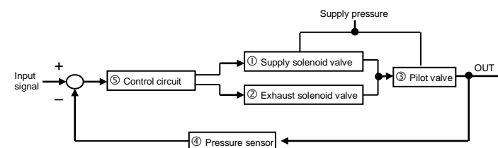
Fig. 1 - Control diagram
